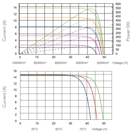
BSM550M10-72HPH
